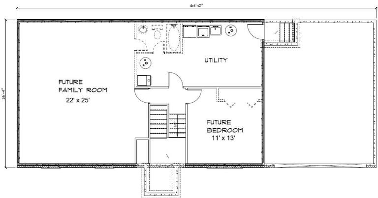
LOWER LEVEL PLAN
